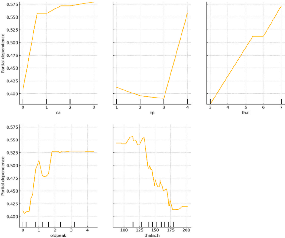
Fig. 5. Partial Dependence Plots generated for random forest model.
