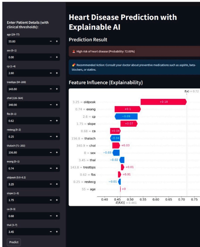
Fig. 10. XAI UI for predicting heart disease.
