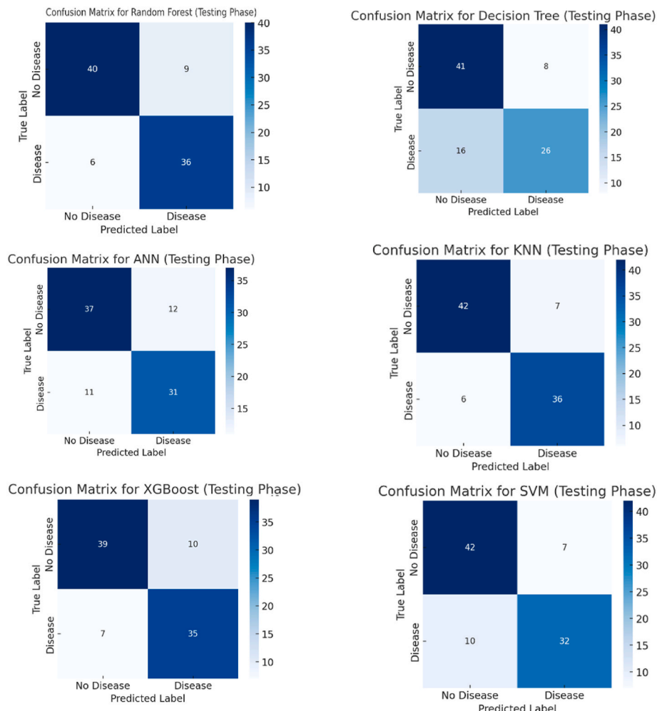
Fig. 3. Confusion matrix of all models for testing.
