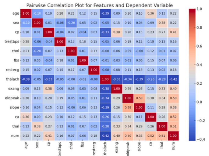
Fig. 2. Pairwise correlation plot for features and dependent variable.
